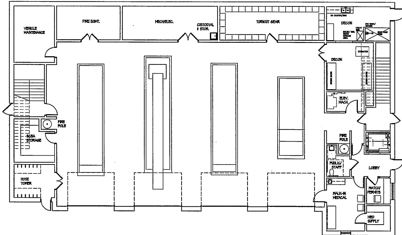
1 FIRST FLOOR - SCHEME F 7,473 GSF 1/16"=1'-0"
